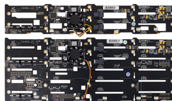
12Gb/s Expander backplane, Optional 6Gb/s backplane
