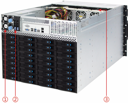
①. CRPS Power Supply ③. Hot-swap Fan Module ②. 2*2.5" HDD/SSD
